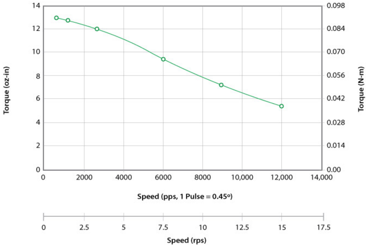
ZN417-11-06 (0.9° Step Motor) 24VDC, 1.12 Amp Peak, Bipolar, 1/2 Stepping
